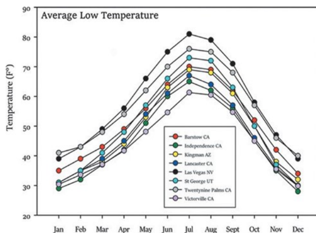
Figure 3 and 4. Average monthly high and low temperatures for cites located in the Mojave Desert. Note the big difference in nighttime low temperatures for Las Vegas vs. Victorville.
