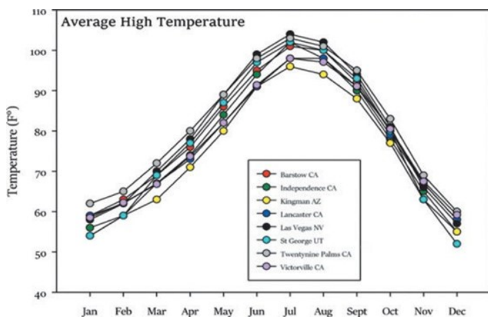
Figure 3 and 4. Average monthly high and low temperatures for cites located in the Mojave Desert. Note the big difference in nighttime low temperatures for Las Vegas vs. Victorville.
