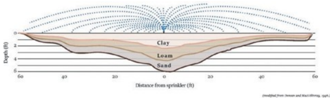
Figure 21. Depth of applied water in the soil by a single sprinkler, based on different soil textures with a single application rate. As the distance from the sprinkler increases, the application of water from a sprinkler decreases. Higher application rates of applied water lead to greater differences in penetration depth of soil moisture. A well-designed sprinkler system spaces sprinkler heads in a manner that achieves overlap to attain maximum uniformity. (Drawing by Nancy Villeda).
