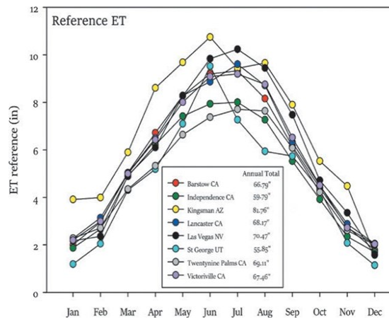
Figure 8. Average monthly reference evapotranspiration (ET) for cities located in the Mojave Desert. ET reference is calculated based on meteorological data, especially solar radiation, temperature, relative humidity, and wind speed. As environmental demand goes up, plant water use typically goes up.
