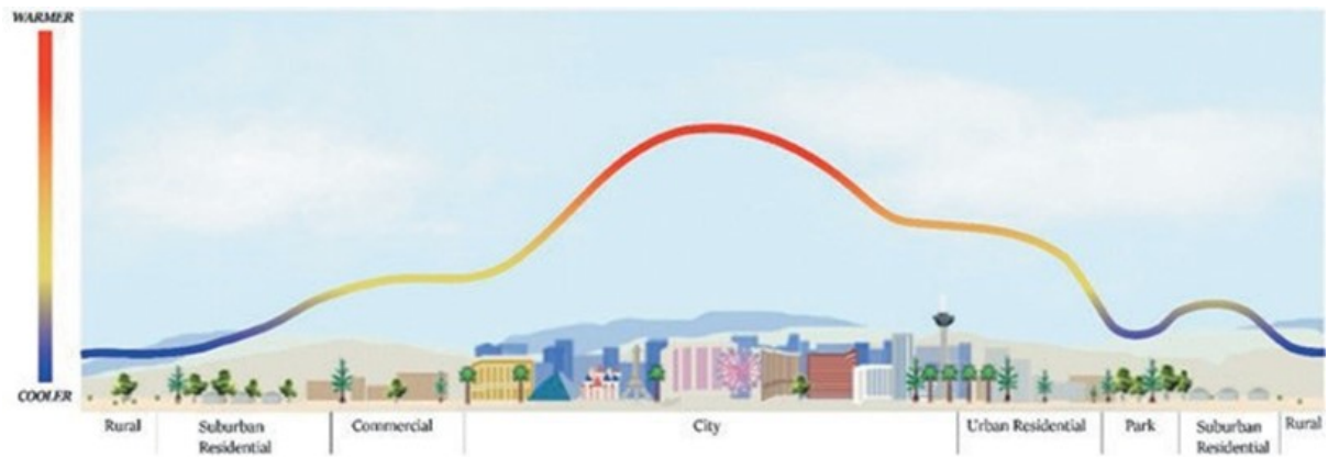
Figure 5. Urban heat island effect with a rise in temperature, compared to rural areas outside of the urban developed area, typically associated with larger metropolitan areas and often accentuated during the night. Asphalt, concrete, and buildings will store heat and release it once the sun goes down. (Drawing by Nancy Villeda).
