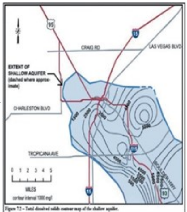
Figure 13. Total dissolved solids (a rough approximation of salinity) contour map of the shallow aquifer in the Las Vegas Valley (permission to use granted by SNWA in 2019).
